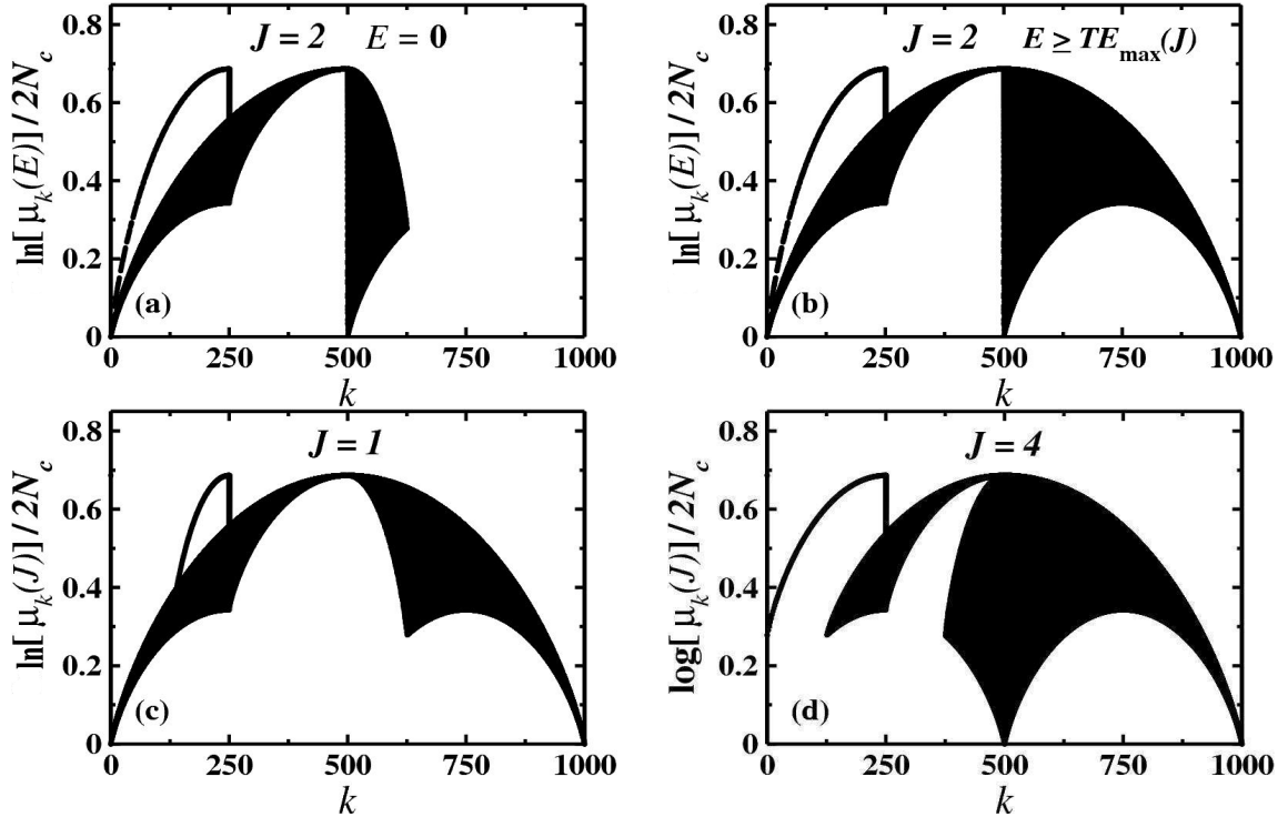
Figure 4.11: (a) \ln[\mu_k(E)]/2N_c for J = 2 and E = E_c(T \neq 0) = 0 , exhibiting the maximum at k = N_c = 500 ; (b) For E \geq E_{T\max}(J) = 6 , the diagram is fulfilled. \ln[\mu_k(J)]/2N_c for E \geq E_{T\max}(J) : for 0 \leq J < 2 , the filled area of the diagram grows up to J = 2 ; for higher values of J , the points at left of the vertical disjoint line ( k = N_c/2 = 250 ) are shifted to the right of this line, as illustrated in (c), (b), and (d), for J = 1 , J = 2 , and J = 4 , respectively. The vertical disjoint lines and curves are explained in the text.
