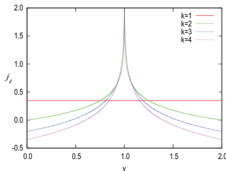
Figure 3.11: Jacobian densities j_\ell as functions of the potential energy v with k = 1, 2, 3, 4 and \Delta = 1 . From Ref. [5]
