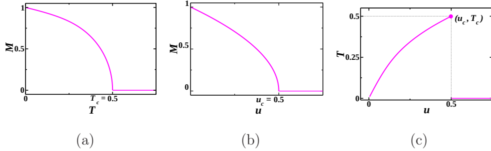
Figure 3.1: Infinite-range XY model: (a) magnetization M vs. temperature T ; (b) M vs. potential energy per particle u ; (c) T vs. u . The system displays a phase transition at u_c = 0.5 and T_c = 0.5 .
