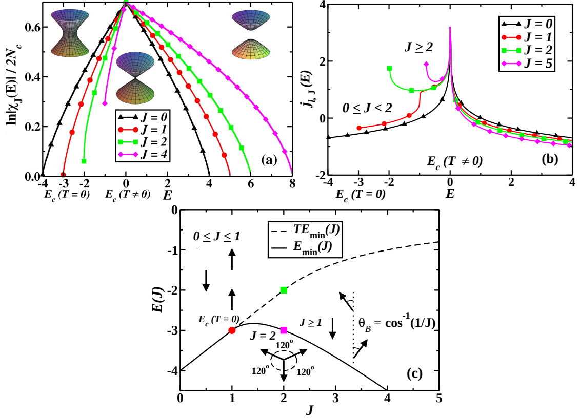
Figure 4.4: Frustrated AB_2 -XY model. (a) Cusp-like pattern exhibited by \ln|\chi_J(E)|/2N_c measured on the surface defined by the intersection of the equipotential surface and the cylinder \mathcal{C}_B (see text). For E < 0 , the equipotential surfaces are one-sheet hyperboloids; at E_c(T \neq 0) = 0, \forall J , we have a cone; and for E > 0 we have two sheet-hyperboloids. For J \geq 2 , \ln|\chi_J(E)|/2N_c is discontinuous at E_{T\min}(E) due to intersection surfaces with zero \chi_J(E) for E_{\min}(J) \leq E < E_{T\min}(J) . The intersection surfaces and \ln|\chi_J(E)|/2N_c vanish at E_{\max} = E_{T\max} = 4 + J . (b) Divergence of j_{l,J}(E) at E_c(T \neq 0) = 0, \forall J . The golden hyperboloid at J = 2 signals the change of the tail curvature of j_{l,J}(E) for E < 0 , associated with the discontinuous behavior shown in (a). (c) E_{\min}(J) and E_{T\min}(J) split at E_c(T = 0) = -3 and J = 1 . For J \geq 2 , there exist intersection surfaces with zero \chi_J(E) in the region limited by E_{\min}(J) and E_{T\min}(J) . The spin structures illustrate the stable phases associated with E_{\min}(J) .
