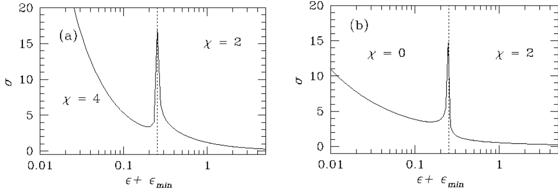
Figure 2.6: The fluctuation \sigma_K of the gaussian curvature of the surfaces \mathcal{F}_\varepsilon and \mathcal{G}_\varepsilon is plotted vs \varepsilon . \sigma is defined in Eq. (2.27), \varepsilon is shifted by \varepsilon_{\min} = 0.25 for reasons of clarity in the presentation. (a) refers to \mathcal{G}_\varepsilon and (b) refers to \mathcal{F}_\varepsilon . The cusps appear at \varepsilon = 0 where the topological transition takes place for both \mathcal{F}_\varepsilon and \mathcal{G}_\varepsilon . From Ref. [12].
