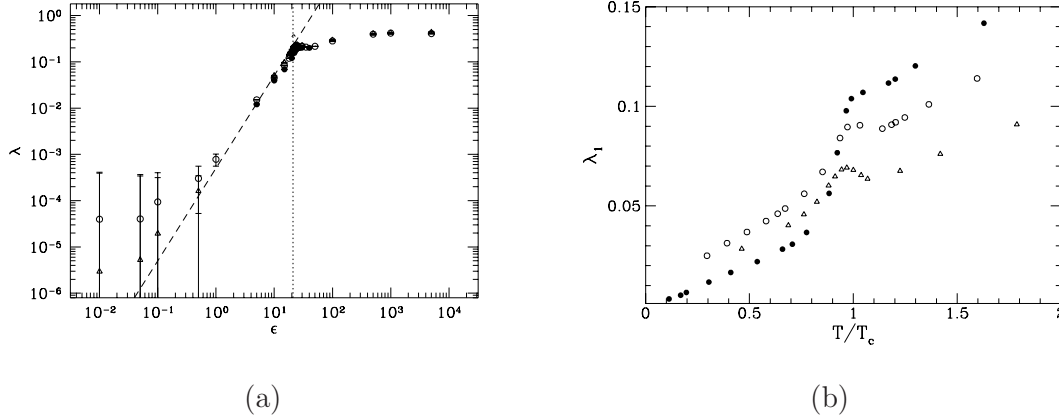
Figure 2.3: (a) Lyapunov exponent \lambda vs. the energy per particle \varepsilon , for the two-dimensional O(1) \varphi^4 model, with N = 100 (solid circles), N = 400 (open circles), N = 900 (solid triangles), and N = 2500 (open triangles), respectively. \varepsilon_c is marked by a dotted line, and the dashed line is the power law \varepsilon^2 . (b) \lambda vs. the temperature T for the three-dimensional \varphi^4 model. Full circles correspond to the O(1) (scalar) case, open circles to the O(2) case, and open triangles to the O(4) case. From Ref. [12].
