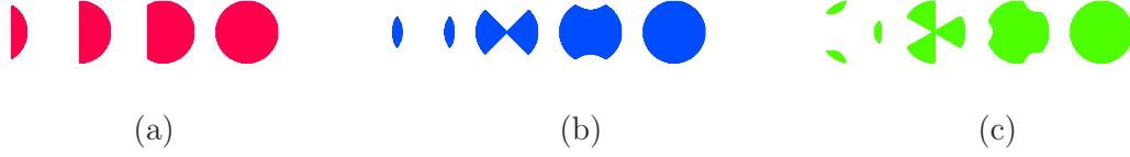
Figure 3.10: The submanifolds \mathcal{M}_v for v = 0.5\Delta, \Delta, 1.5\Delta, 2\Delta (from left to right). (a) For k = 1 , all the submanifolds are topologically equivalent to a single disk. (b) In the case k = 2 , for v < v_c = \Delta the submanifolds are topologically equivalent to two disconnected disks, while for v > v_c are equivalent to a single disk. (c) In the case k = 3 , for v < v_c = \Delta the submanifolds are topologically equivalent to three disconnected disks, while for v > v_c are equivalent to a single disk. From Ref. [32]
