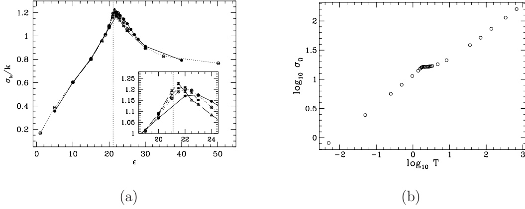
Figure 2.4: (a) Root mean square fluctuation of the Ricci curvature (Eisenhart metric) \sigma_k , divided by the average curvature k_0 , for the two-dimensional O(1) \varphi^4 model. The inset shows the transition vicinity. Symbols as in Fig. 2.3. From Ref.[22, 3, 1]. (b) Curvature fluctuations \sigma_k vs. the temperature T for the two-dimensional O(2) \varphi^4 model, computed on a square lattice of 30 \times 30 sites. The critical temperature T_c of the BKT transition is at T_c \simeq 1.5 . From Refs. [12, 3, 1].
