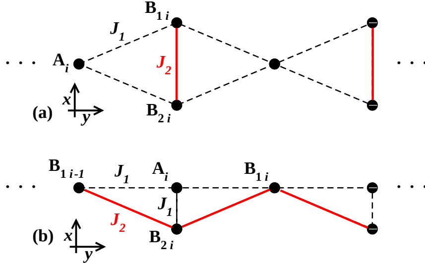
Figure 4.1: Frustrated AB_2 chain: only first-neighbor competing AF couplings, J_1 and J_2 , are indicated. (b) Distinct chain with three-site unit cell topology (see text).
