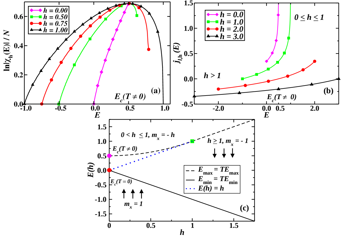
Figure 4.8: Standard Infinite-range XY model in a field. (a) \ln|\chi_h(E)|/N : cusp-like pattern (discontinuity) at (for) h = 0 ( 0 \leq h < 1 ). (b) Divergence of j_{I,h}(E) for 0 \leq h \leq 1 ; the PT occurs at E_c(T \neq 0) = 1/2 and h = 0 . The divergence is suppressed for fields beyond the spin saturation field predicted by E_{T_{\max}} at h = 1 . (c) h -Dependent energies and magnetization.
