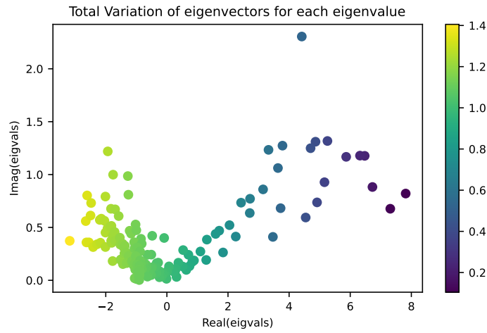
Figure 44 – Total variation of eigenvectors of the symmetric graph adjacency matrix.
