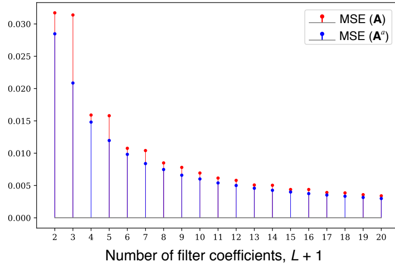
Figure 23 – Minimum approximation (mean squared) errors, for different values of L , between the ideal LPF and the filters designed by using the fractional graph shift operator \mathbf{A}^a and the non-fractional operator \mathbf{A} .
