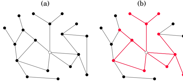
Figure 7 – (a) A graph and (b) the set of vertices \mathcal{N}(i, 2) shown in red, with v_i being depicted in white. The edges linking v_i to the elements in \mathcal{N}(i, 2) are also highlighted in red.
