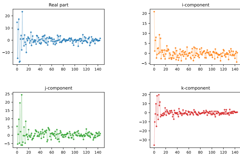
Figure 38 – Spectrum of the quaternion graph signal, defined over the vertices of the graph with Hermitian adjacency matrix.
