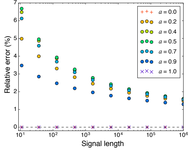
Figure 16 – Percent error (normalized by the energy of \mathbf{h}_{LPF} ) of \mathbf{h}_a related to \mathbf{h}_{LPF} , for different (odd) values of N and the fractional shift parameter a .
