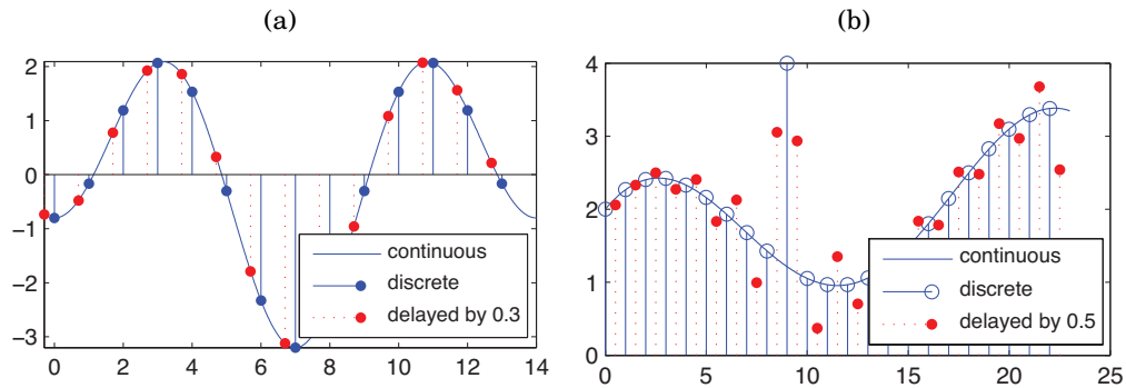
Figure 15 – Fractional shift for a signal (a) without and (b) with abrupt variations (discontinuities).
