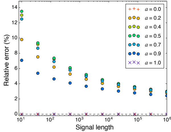
Figure 17 – Relative mean error between \mathcal{Re}\{\mathbf{h}_a\} and \mathbf{h}_{LPF} for N even, in terms of the fractional shift parameter a .
