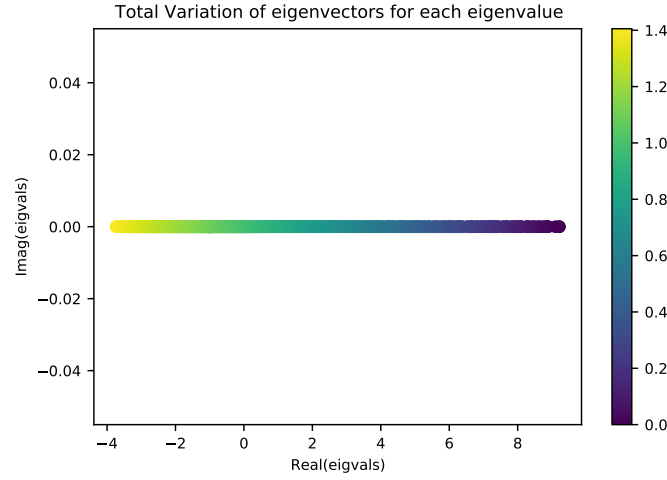
Figure 49 – Total variation for each eigenvector of the (Hermitian) adjacency matrix of the US graph.
