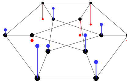
Figure 5 – Example of signal defined over a graph. The height of the vertical bars indicate the value of the signal samples, which are indexed by the graph vertices. The graph edges capture similarity relations between samples. How could one define spectral analysis and processing techniques in such a signal domain?
