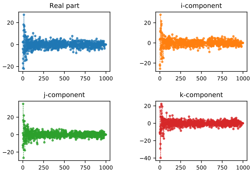
Figure 50 – US graph signal spectrum.
