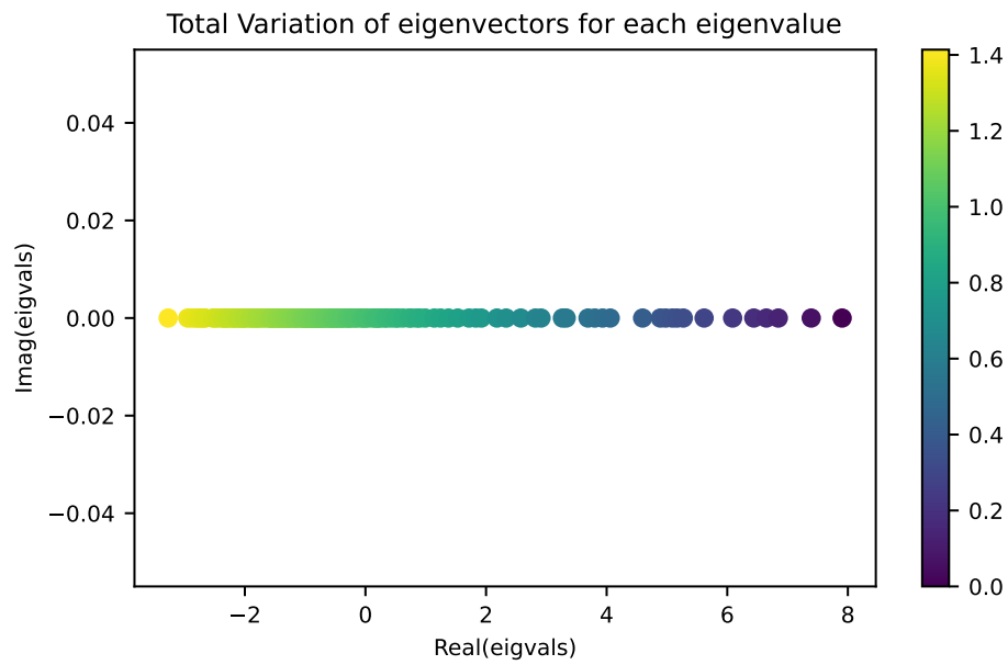
Figure 40 – Total variation of the eigenvectors of the Hermitian graph adjacency matrix, for each respective eigenvalue.
