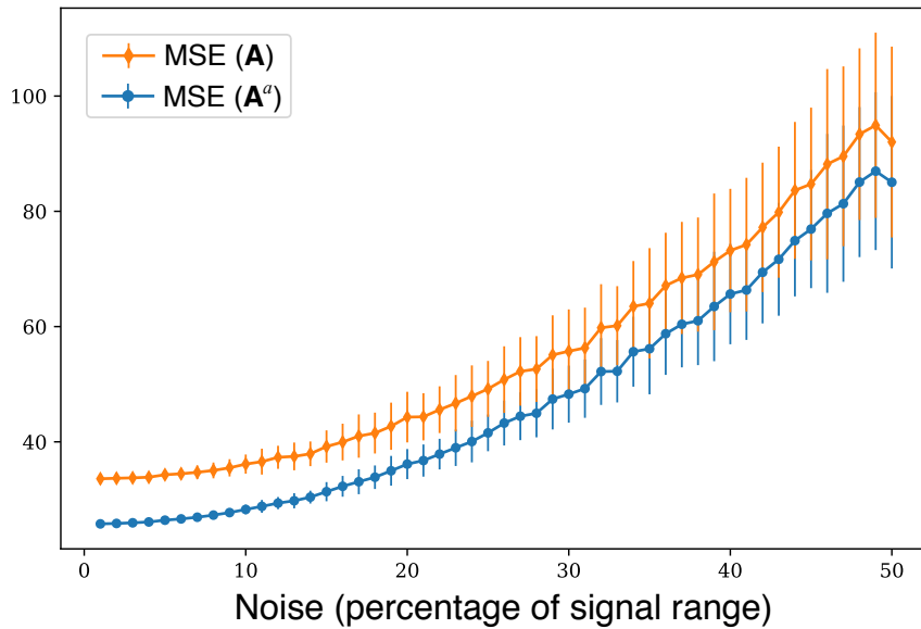
Figure 25 – Reconstruction (mean squared) errors after a noise removal procedure is performed by using graph filters with L + 1 = 10 coefficients and designed from \mathbf{A} and \mathbf{A}^a , a = 0.855 .
