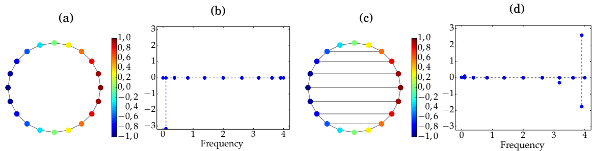
Figure 9 – The same signal defined over two similar graphs, one of them being (a) the undirected ring graph. In (b) and (d) are depicted the Fourier spectra of the signals in (a) and (c), respectively.
