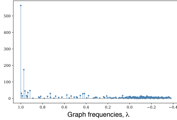
Figure 21 – Magnitude of the graph Fourier transform of the signal in Fig 20. The graph frequencies correspond to the eigenvalues of \mathbf{A} ; low (resp. high) graph frequencies are associated with higher (resp. lower) eigenvalues.
