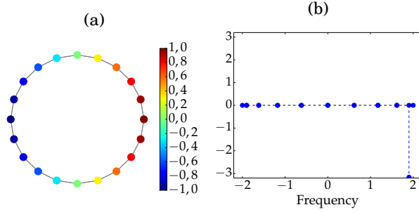
Figure 10 – (a) Signal defined over an undirected ring graph and (b) its spectrum. The frequencies are indicated by the eigenvalues of the adjacency matrix.
