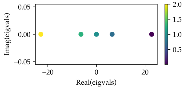
Figure 34 – Graph total variation (pseudocolor scale) of the normalized eigenvectors, as a function of their respective eigenvalues.
