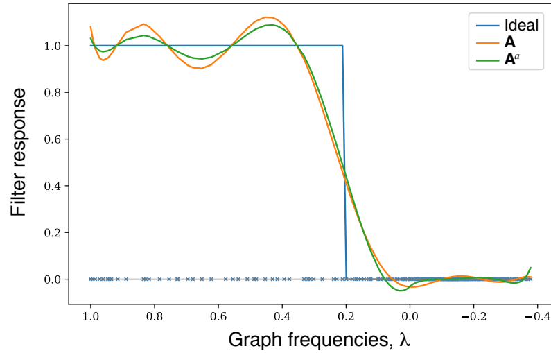
Figure 24 – Ideal filter response superimposed on the responses obtained when \mathbf{A} and \mathbf{A}^a , a = 0.855 , are used to design a filter with L + 1 = 10 coefficients.
