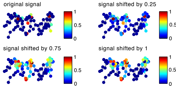
Figure 14 – Fractional shift of a signal, (originally) with 10 non-zero samples, defined on a graph formed by 80 cities of Pernambuco state, Brazil. Note that the shifted signal is similar to the original signal, if a is close to 0, and similar to the unit-shifted signal, if a is close to 1.
