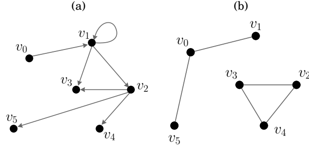
Figure 6 – Examples of (a) directed and (b) undirected graphs, defined over the same vertex set.
