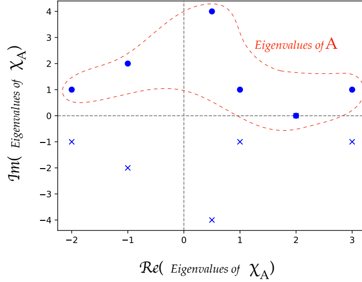
Figure 3 – Standard eigenvalues of a quaternion matrix \mathbf{A} , indicated as a subset of the eigenvalues of the complex adjoint matrix.
