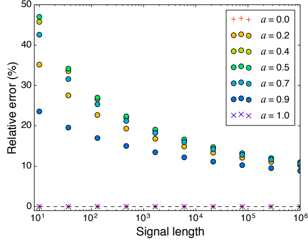
Figure 18 – Modulus of the relative mean error between \mathbf{h}_a and \mathbf{h}_{LPF} for N even, in terms of the fractional shift parameter a .
