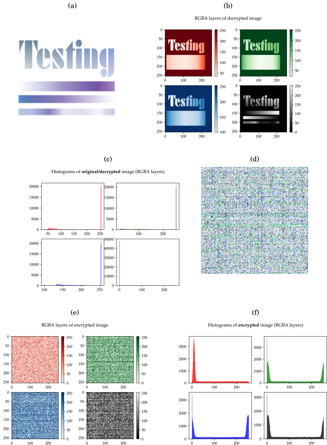
Figure 31 – (a) Test image in PNG format, with 256 \times 256 pixels. (b) Color and opacity layers of the decrypted image (which coincides with the original in (a)). (c) Histograms of each layer of the decrypted image. (d) Encrypted image, in PNG format. (e) Color and opacity layers of the encrypted image. (f) Histograms of each layer of the encrypted image.
