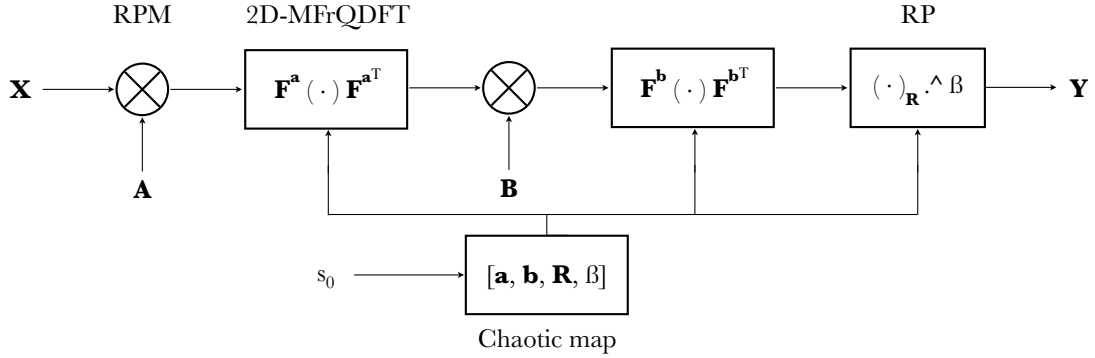
Figure 28 – Proposed encryption scheme, exploring the 2D-MFrQDFT.
