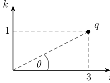
Figure 2 – Representation of \lambda = 3i + k in the ik plane.
