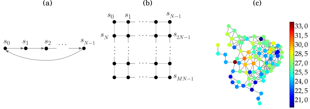
Figure 8 – Examples of depictions of graph signals over (a) a directed ring graph, (b) an undirected regular grid graph and (c) a graph of cities from the Brazilian Northeastern region, over which was defined a signal of temperature measurements from February 1 st of 2012, retrieved from the Banco de Dados Meteorológicos para Ensino e Pesquisa (BDMEP, freely translated as Meteorological Database for Teaching and Research), available at: http://www.inmet.gov.br/portal/index.php?r=bdmep/bdmep .
