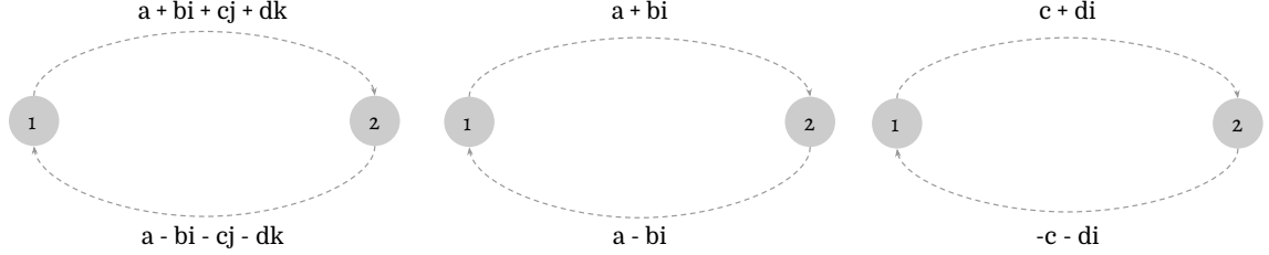
Figure 33 – Illustration of two connected vertices in a graph with Hermitian adjacency matrix (left-hand side). In the center and on the right, respectively, are displayed the edges created by the simplex and perplex parts of the adjacency matrix.
