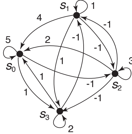
Figure 19 – Directed graph used to illustrate how the corresponding fractional shift operator can be computed and represented in polynomial form.
