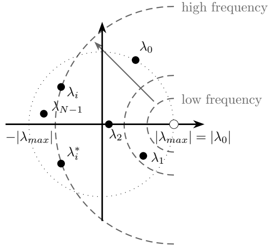
Figure 11 – Frequency ordering of graph signals, from low to high frequencies, in the complex plane.
