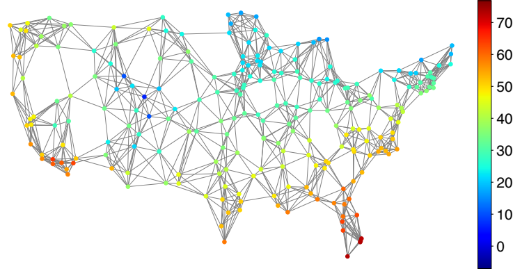
Figure 20 – Graph of a network formed by 230 weather stations measuring the temperature across the United States. The snapshot of all measurements taken on February 1 st , 2003 is the corresponding graph signal.
