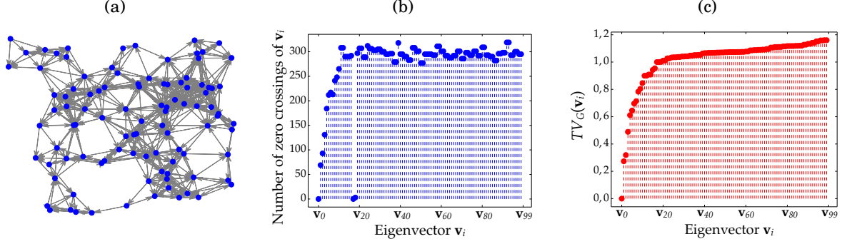
Figure 12 – (a) Directed sensor graph, with N = 100 vertices and no loops or multiple edges. (b) Number of zero crossings and (b) total variation of the eigenvectors (\mathbf{v}_i)_{i=0,\dots,N-1} of the adjacency matrix \mathbf{A} of the graph in (a), ordered so that the respective eigenvalues appear from the closest to the farthest from the real point |\lambda_{max}| in the complex plane. That is, according to (87) and Fig. 11, the eigenvectors are disposed in ascending order of frequency.
