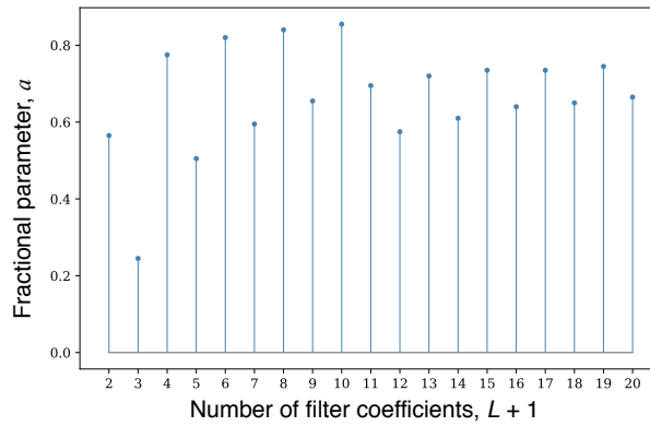
Figure 22 – Fractional parameters providing the minimum approximation errors, for different values of L , between the ideal LPF and the filter designed by using the fractional graph shift operator \mathbf{A}^a .
