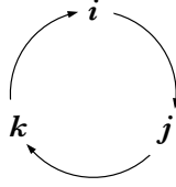
Figure 1 – Illustration of the multiplication rule between the imaginary units i , j and k .
