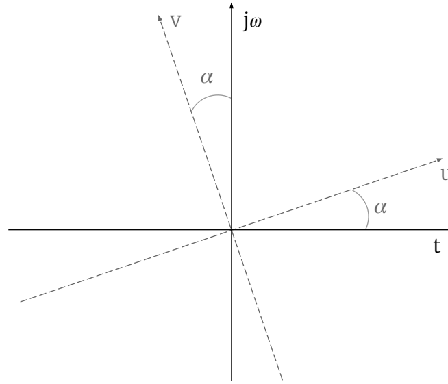
Figure 4 – Illustration of the FrFT property of rotation in the time-frequency plane.
