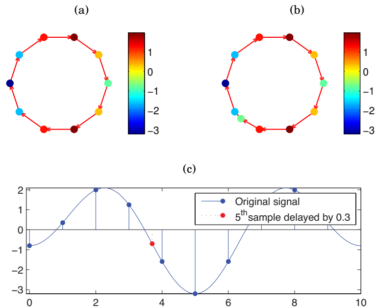
Figure 13 – Fractional shift by a = 0.3 of a sample of a signal on a directed ring graph with unit weights. (a) Original signal on a directed ring graph. (b) Graph in which the 5 th sample delayed by a = 0.3 appears as an interpolated sample between the 4 th and the 5 th samples of the original signal. (c) Original discrete signal and the delayed sample.
