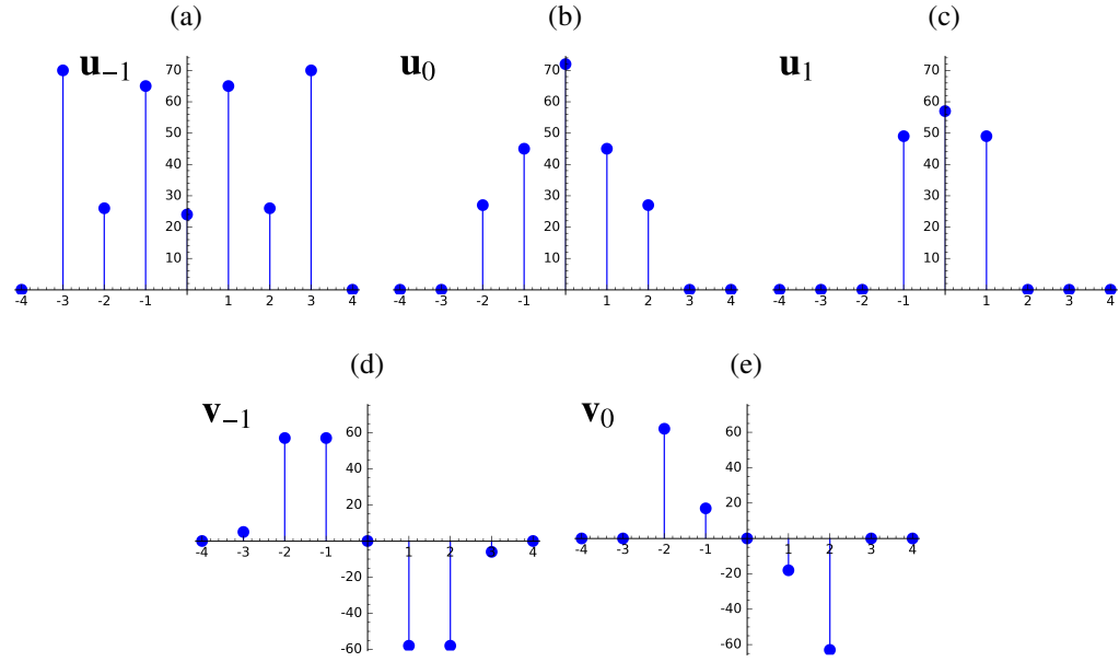
Figura 20 – Vetores: (a) \mathbf{u}_{-1} , (b) \mathbf{u}_0 , (c) \mathbf{u}_1 , (d) \mathbf{v}_{-1} , e (e) \mathbf{v}_0 .
