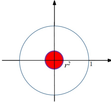
Figure 6: Support of u_\varepsilon^r .
