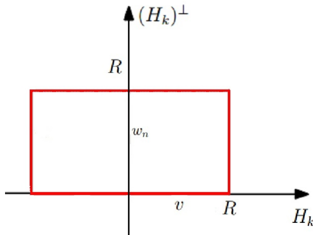
Figure 2: Q := \{v + sw_n : v \in H_k, \|v\| \leq R \text{ and } 0 \leq s \leq R\} .
