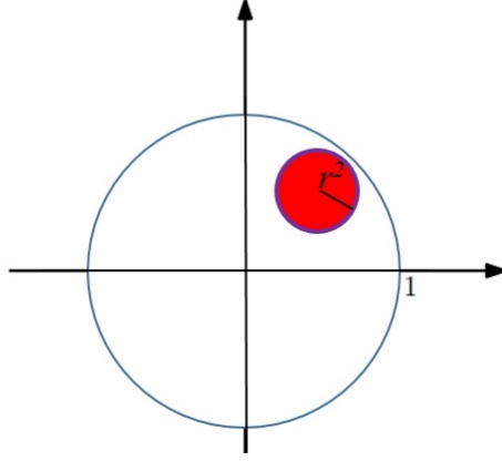
Figure 3: Support of z_n^r .
