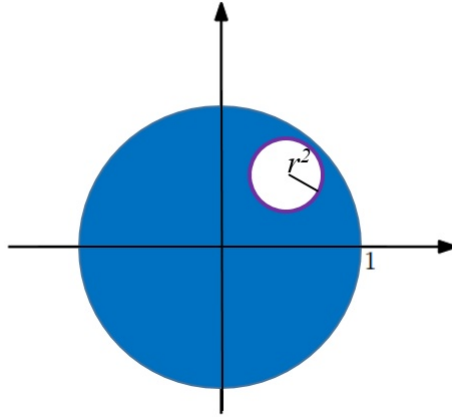
Figure 4: Support of v \in H_k^r is a subset of B_1 \setminus B_{r^2} .
