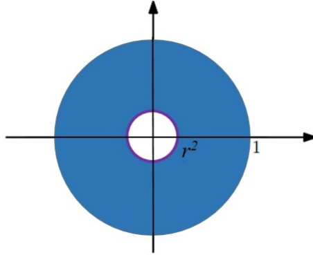
Figure 5: Supports of \psi_r and f_r .
