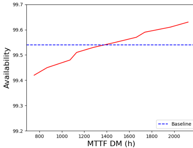
Figure 31 – Sensitivity of system availability with respect to MTTF_{DM} (device manage component failure)
