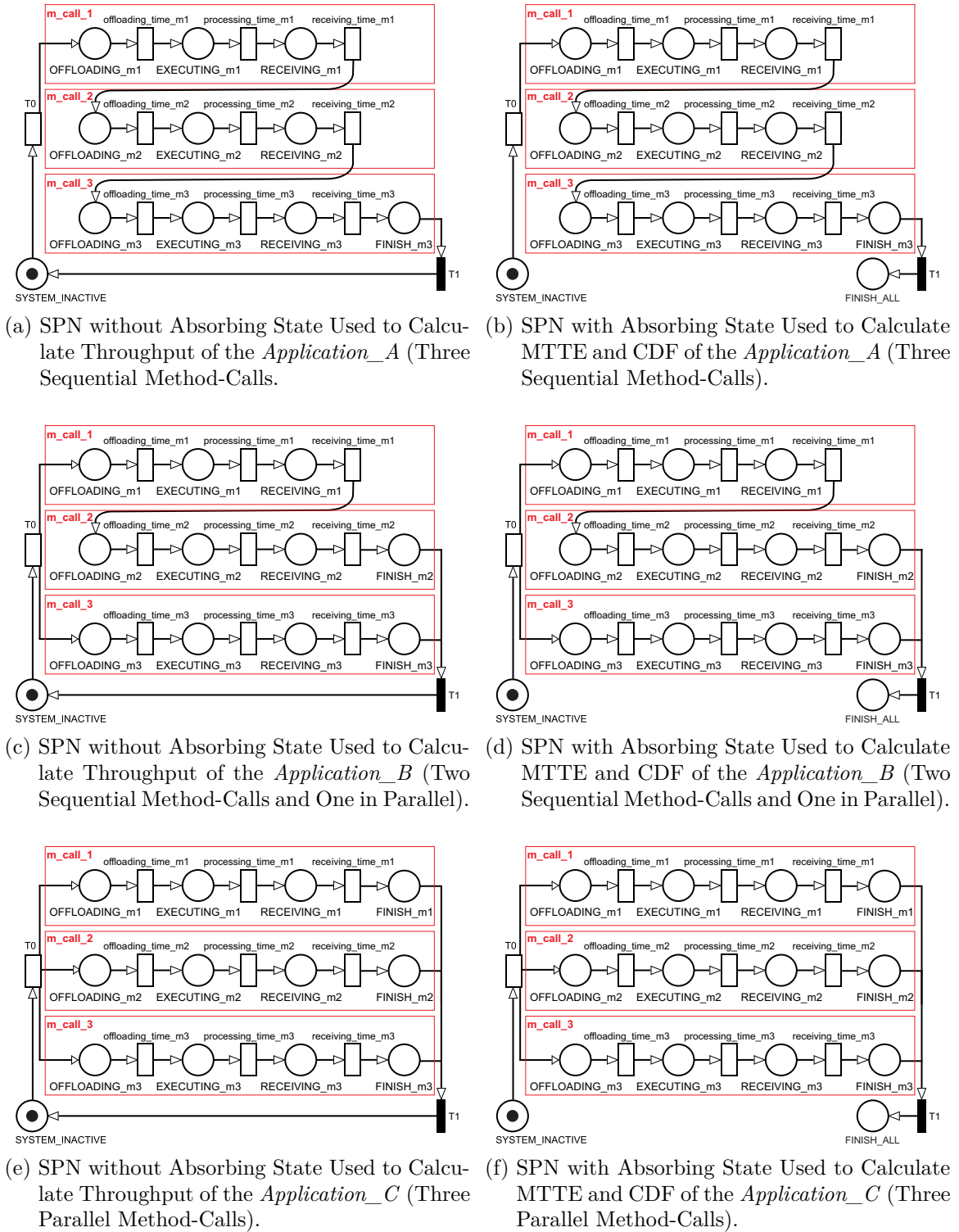
Figure 33 – SPNs Representing Offloadable Method-Calls
