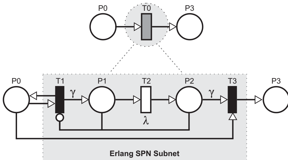
Figure 13 – Erlang Distribution SPN Subnet
