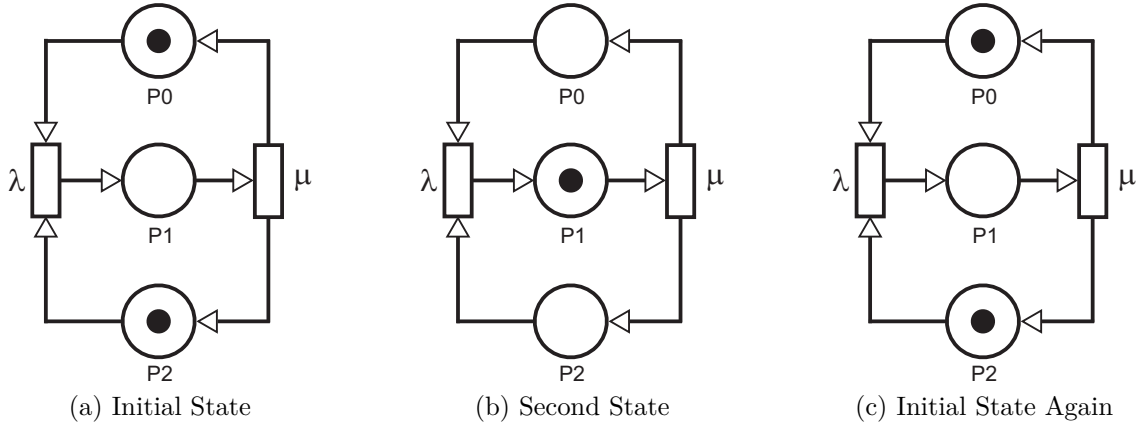
Figure 10 – Example of a basic SPN
