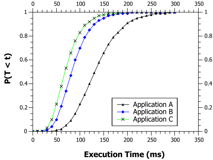
Figure 34 – Example of CDF based on SPN
