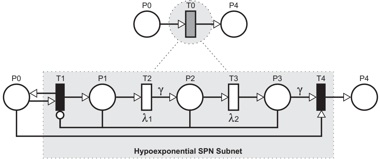
Figure 15 – Hypoexponential Distribution SPN Subnet
