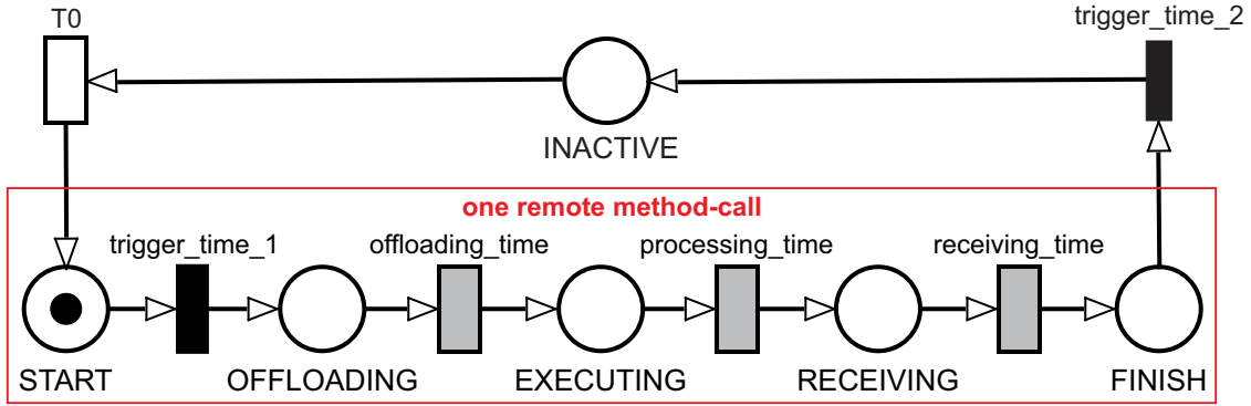
(b) SPN without Absorbing State Used to Calculate Throughput of an Application With One Offloadable Method-Call.
