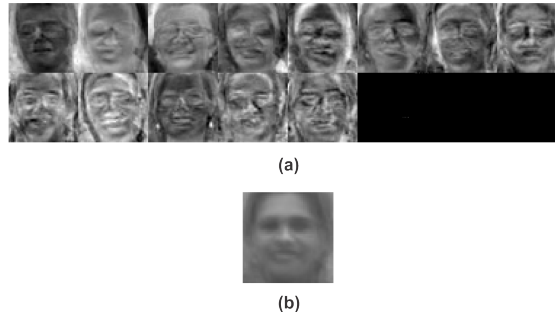
Figure 18 – (a) Thirteen eigenfaces calculated considering the faces of Figure 17; (b) The average face.
