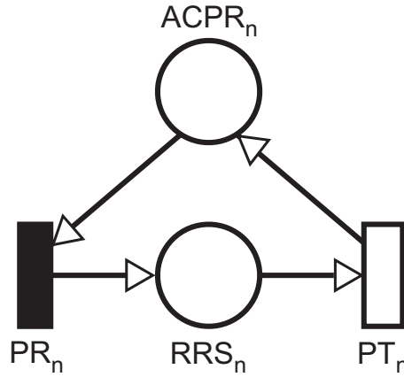
Figure 38 – SPN Subnet Representing a Type of Service Instances
