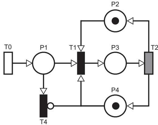
(a) An SPN Model with a Non-Exponential Timed Activity.
