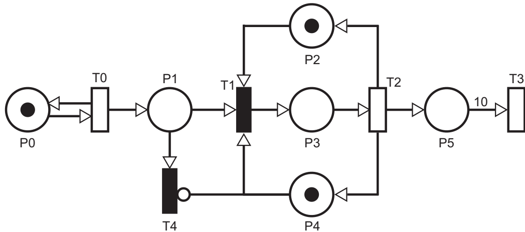
Figure 12 – An Example of an SPN model
