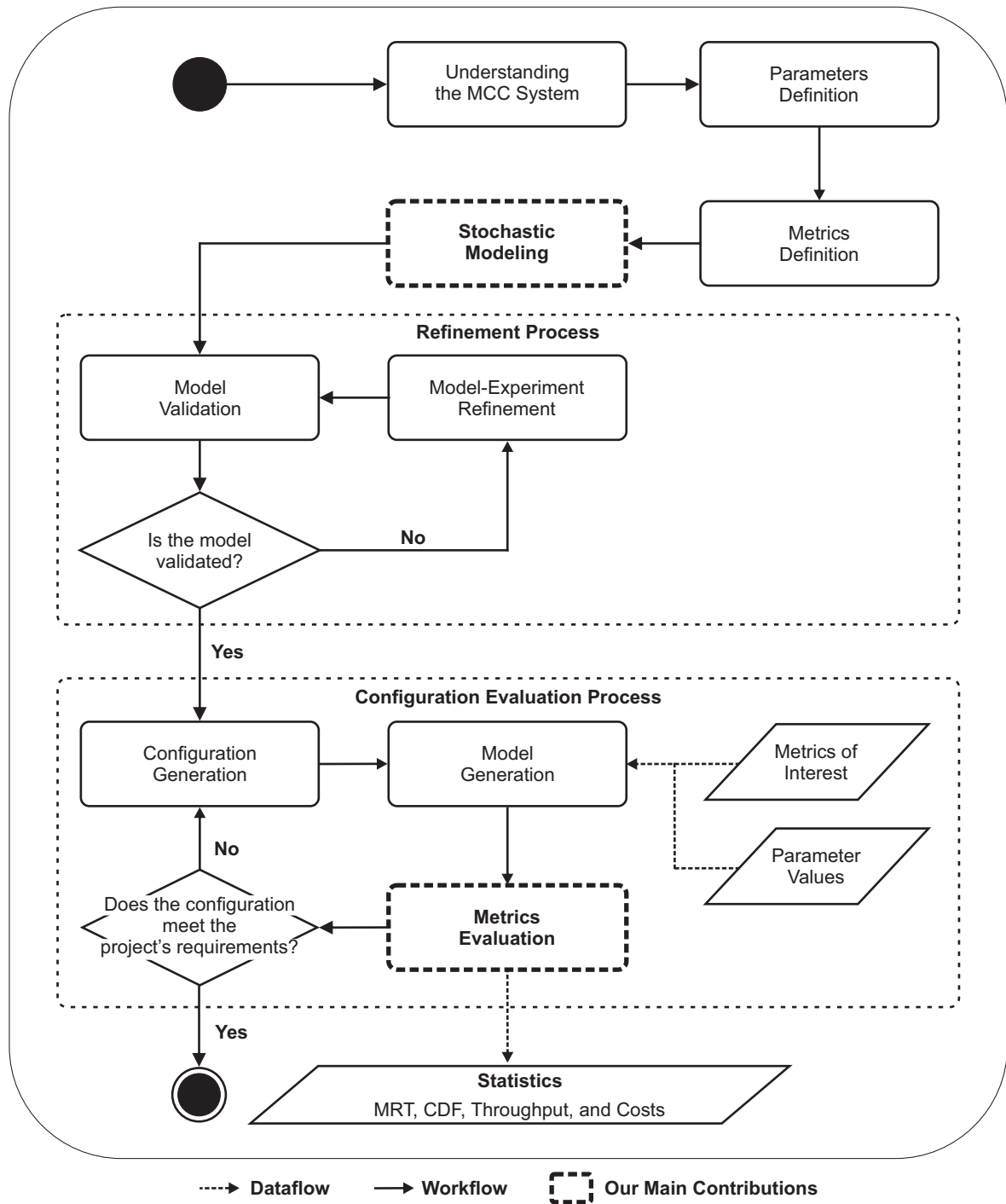
Figure 25 – Steps of the Methodology for Planning MCC Systems in Public Clouds
