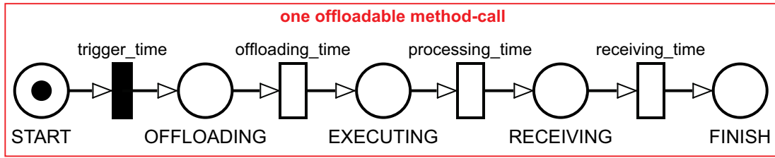
Figure 63 – SPN with Absorbing State Used to Calculate MTTE of an Application With Only One Offloadable Method-Call
