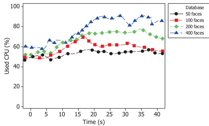
Figure 22 – Mobile Device CPU Profiling
