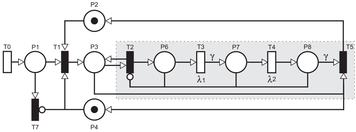
(b) An SPN Model with a Hypoexponential Subnet.
