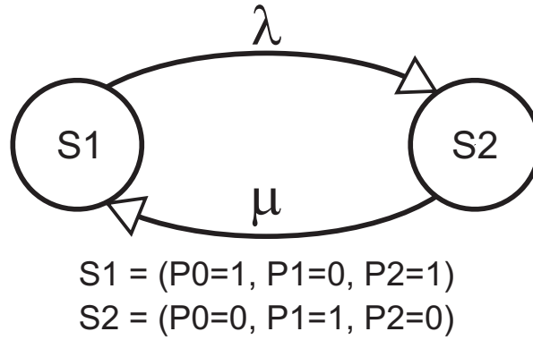
Figure 11 – CTMC Related to the State Space of the SPN Presented in Figure 10
