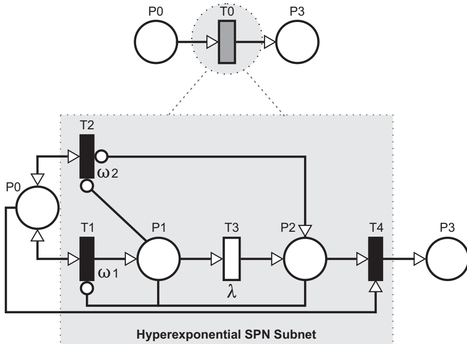
Figure 14 – Hyperexponential Distribution SPN Subnet
