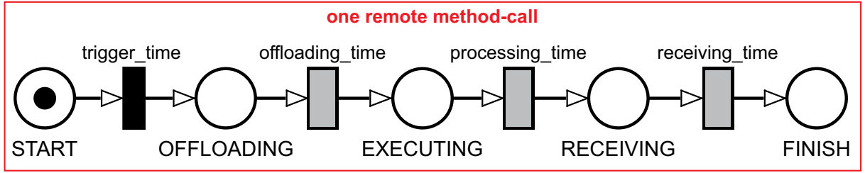
Figure 31 – Basic SPN Representation of One Application with Only One Offloadable Method-Call Using Absorbing State
