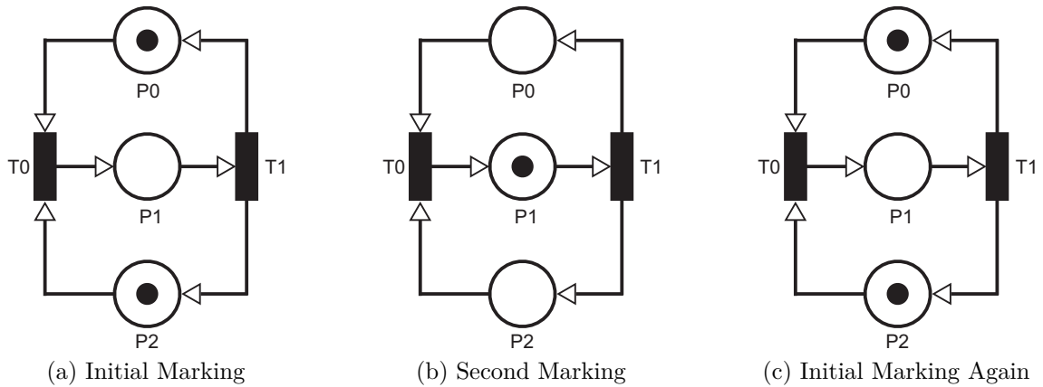
Figure 8 – Example of a Petri Net
