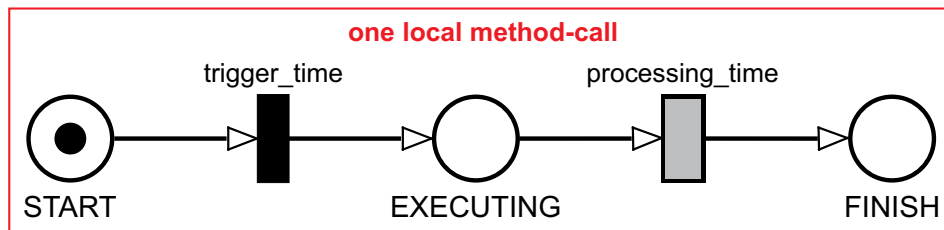
Figure 30 – Basic SPN Representation of One Application with Only One Local Method-Call Using Absorbing State
