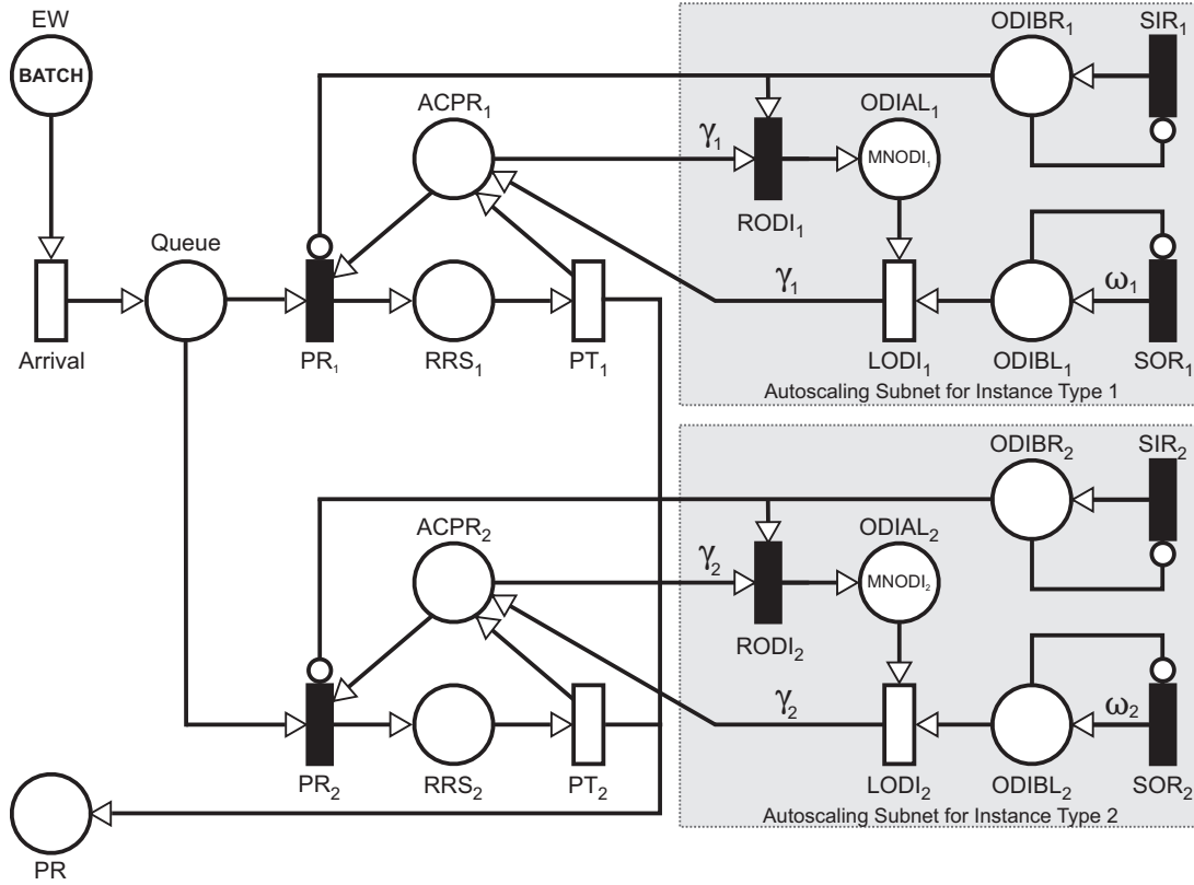
Figure 58 – Public Cloud MCC Infrastructure Model Refined to Calculate CDFs and MTTAs
