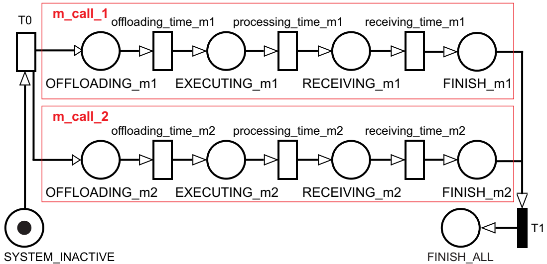
Figure 43 – SPN Model Representing the Method processImages()
