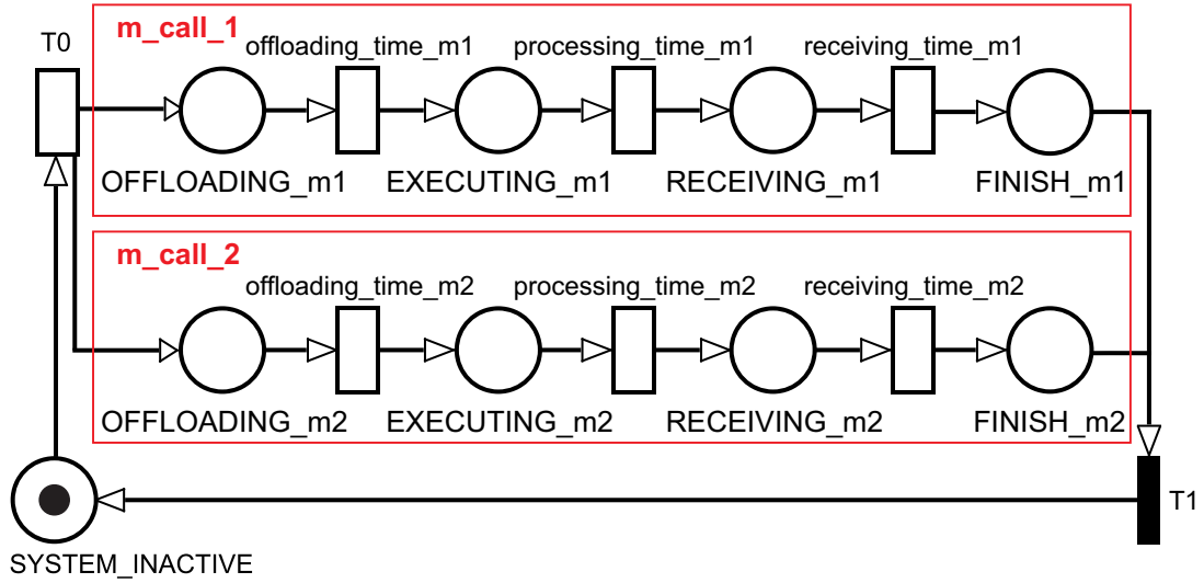
Figure 48 – SPN Used to Calculate Throughput of an Application With Two Parallel Method-Calls
