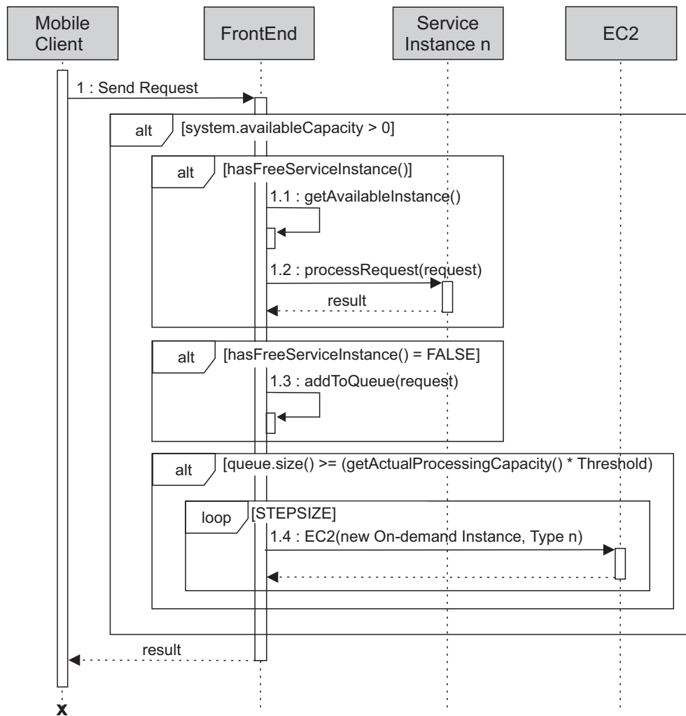
Figure 29 – Sequence Diagram Depicting the Front-end Behaviour When a Request Arrives in the System
