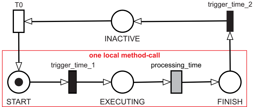
(a) SPN without Absorbing State Used to Calculate Throughput of an Application With One Local Method-Call.
