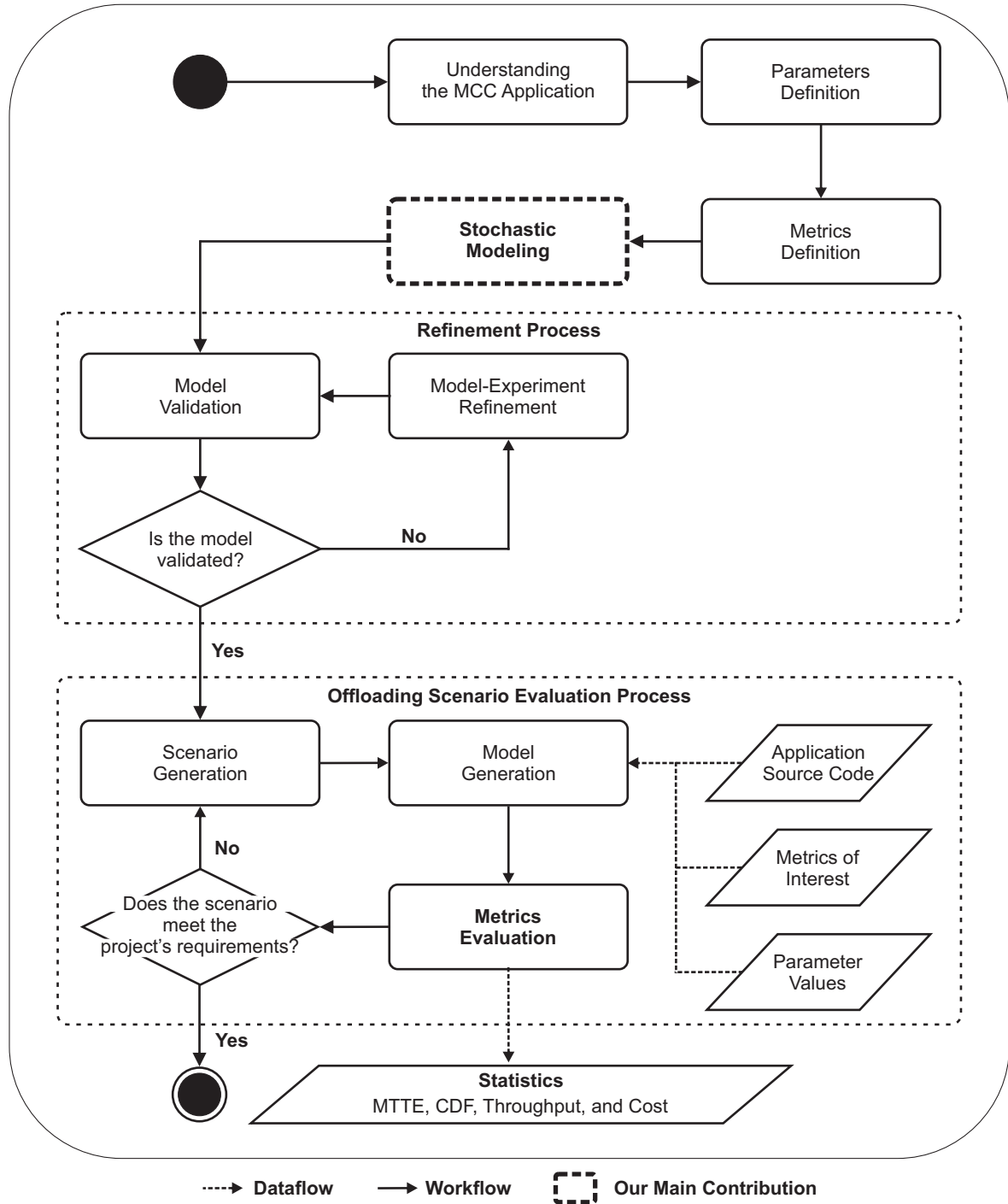
Figure 20 – Steps of the Methodology for Evaluating MCC Applications' Offloading
