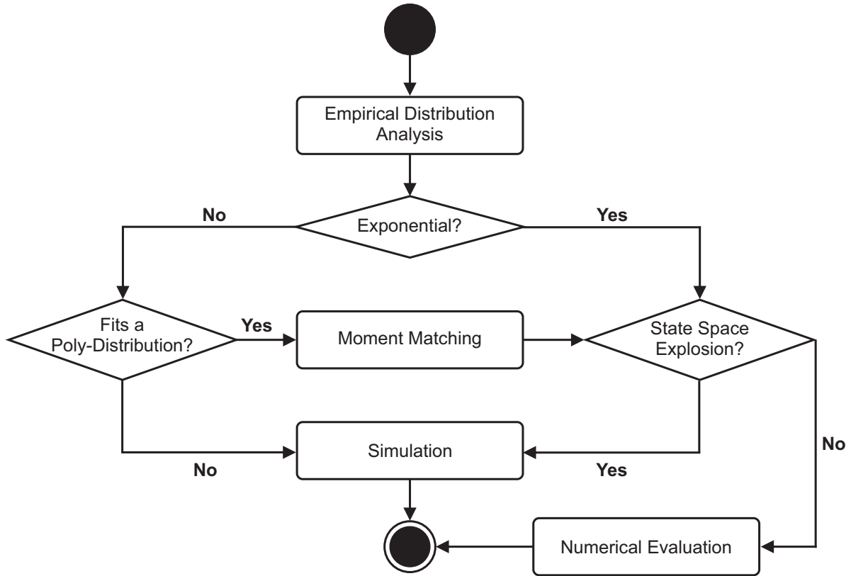
Figure 24 – Decision Process for Metrics Evaluation
