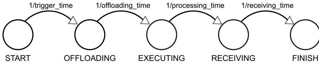
Figure 32 – CTMC of an Application with Only One Offloadable Method Call With Absorbing State
