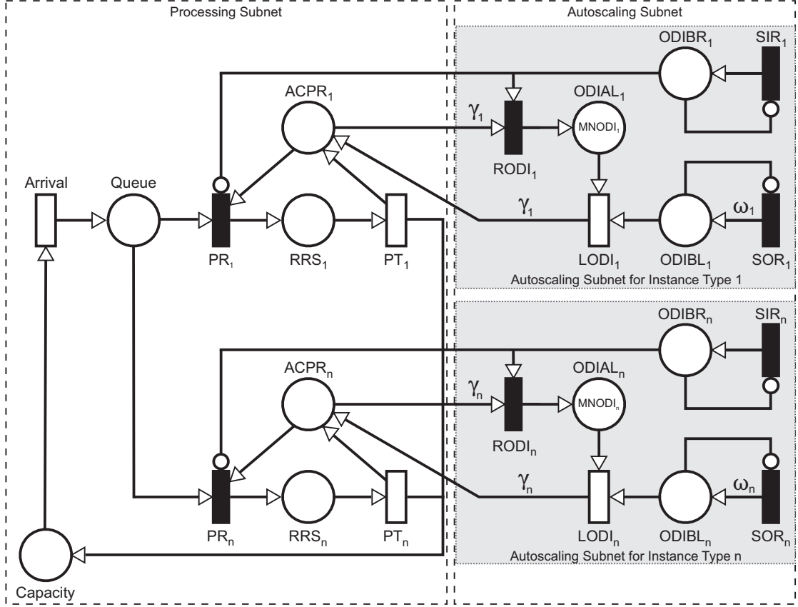
Figure 36 – Public Cloud MCC Infrastructure Model
