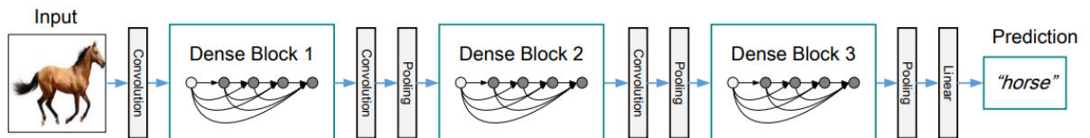
Figure 15: DenseNet architecture (Huang et al. , 2017)
