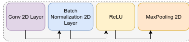
(a) Custom layer used on MNIST CNN Model.
