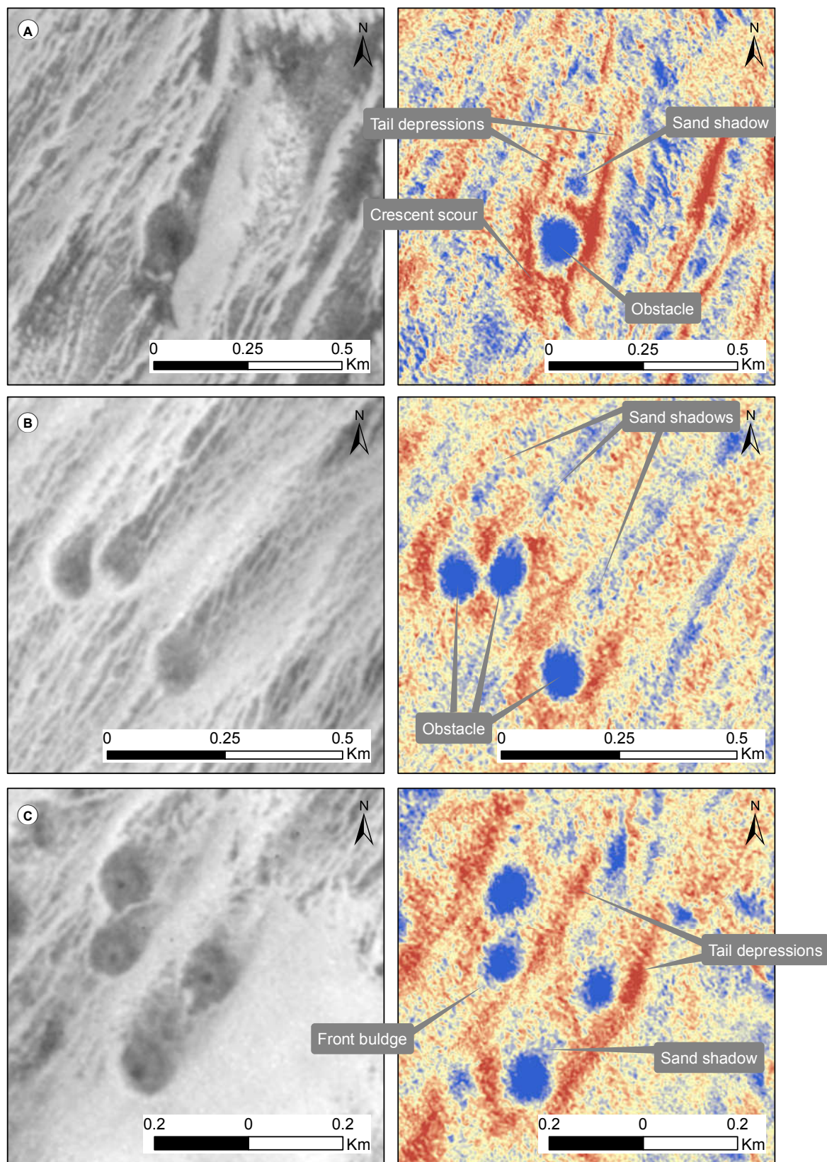
Fig. 15: Examples of comet marks and their individual characteristic forms, as first described by Werner et al. (1980). On the left-hand column, LiDAR reflectance images. On the right side, BPI < 70 \text{ m} > images.
