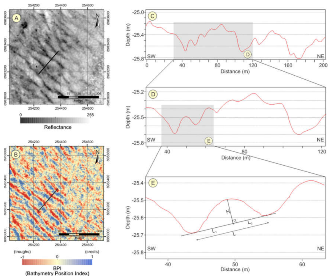
Fig. 6: (A) LiDAR reflectance image example in the dune field off Porto de Pedras; (B) BPI < 70 \text{ m} > image of the same example; (C) bathymetric profile indicated in A and B; (D) first order subaqueous dunes; and (E) second order subaqueous dunes. (The black line in (A) and (B) indicates the location of the bathymetric profile shown in (C)).
