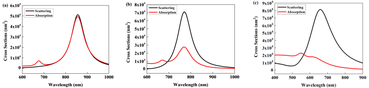
Figure 34- Nanoshells scattering and absorption cross sections with core radius 42 nm and shell thickness 5 nm (a), 10 nm (b) and 20 nm (c), respectively.
