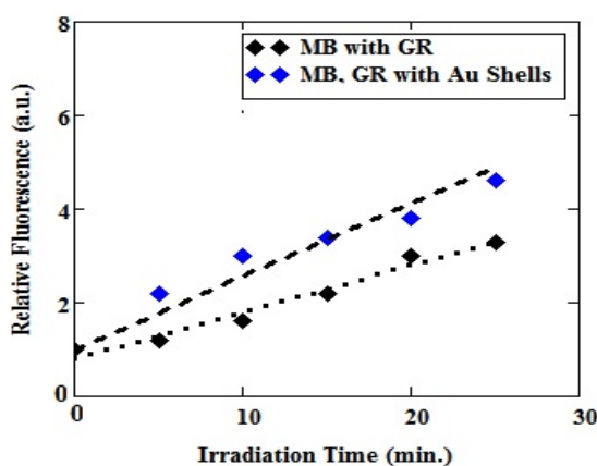
Figure 40- Fluorescence intensity ratio of GR with several irradiation time for MB solution with and without Au nanoshells.
