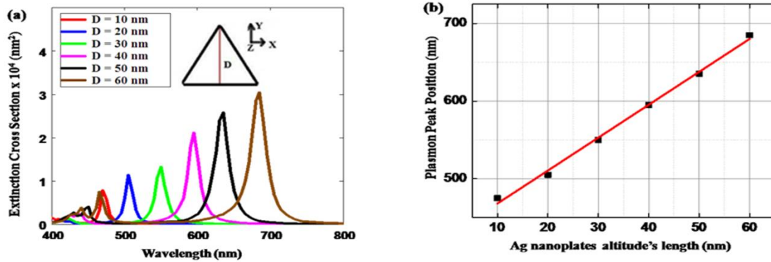
Figure 23- Simulated LSPR extinction spectra of AgNPLs with different altitude lengths, t = 10 nm and n = 1.33 (a). Plasmon peak positions for various AgNPLs altitude lengths (b).
