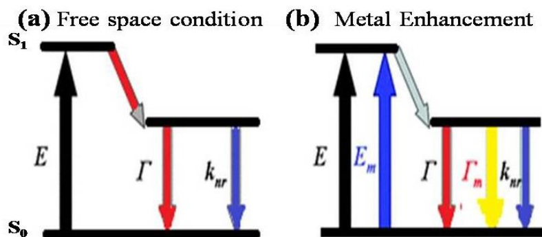
Figure 13- Jabłoński diagram with and without (free space) metal plasmon resonance. E_m and E indicate the excitation rate with metal and in free space respectively. While \Gamma_m and \Gamma depicts respectively radiative rate in proximity of metal and in free space, k_{nr} is the non-radiative decay rate.
