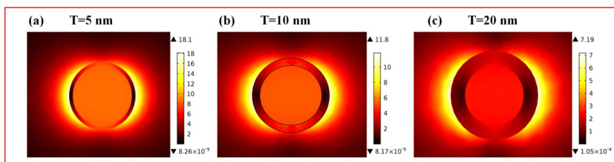
Figure 35- The normalized electric field distribution at XY plane of silica core/Au shells with the thickness (a) T = 5 nm, (b) T = 10 nm, and (c) T = 20 nm corresponded to the fields at extinction spectral peaks 854 nm, 714 nm and 650 nm plasmonic wavelengths respectively.
