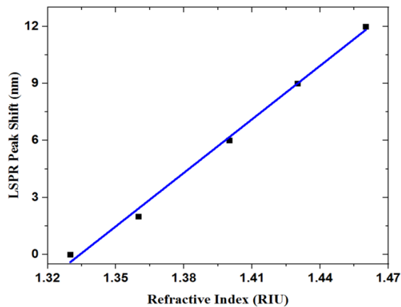
Figure 10- The plasmon peak wavelength shift for different refractive index medium obtained experimentally.
