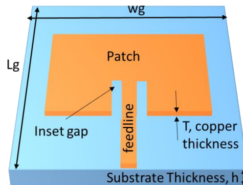
Figure 7.3: Inset-Fed Patch Antenna Design
