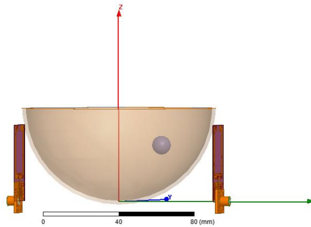
Figure 9.7: Array of Two Antennas at 180^\circ along axes to each other
