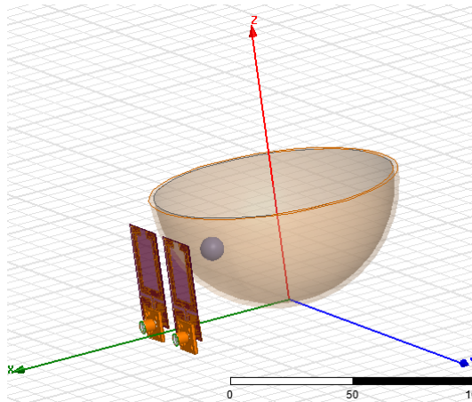
Figure 9.3: Two Antenna at 0^\circ with 30mm Distance Apart
