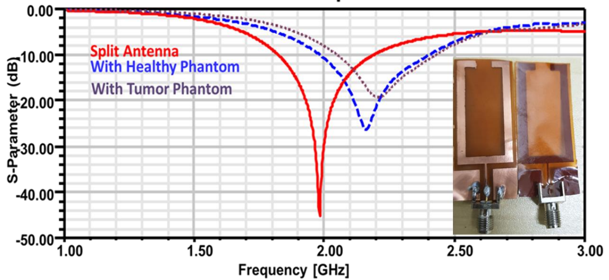
Figure 9.11 Response of an S11 parameter of Split Pyralux Polyimide Antenna with healthy and tumor phantom
