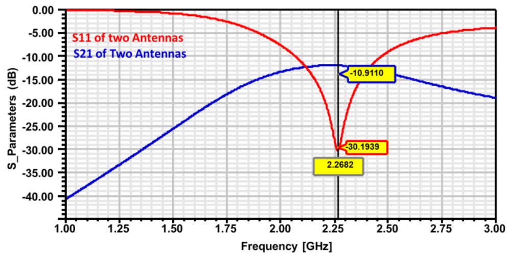
Figure 9.8: Array of Two Antennas at 180^\circ along axes to each other
