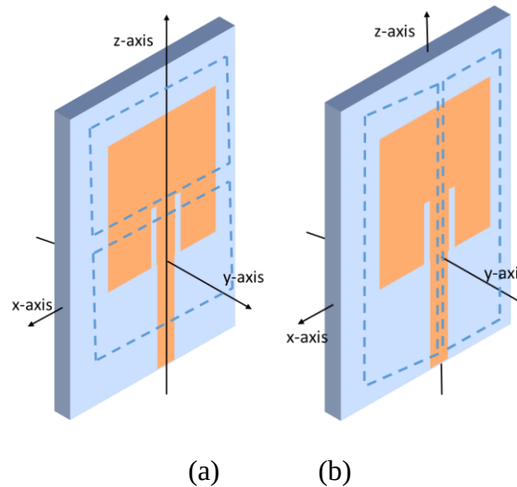
Figure 7.11: Propagation of radiation in Rectangular Patch Antennas
